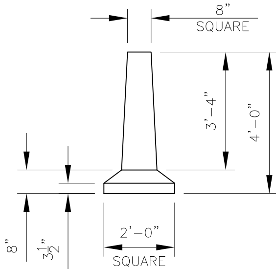
ELEVATION VIEW
