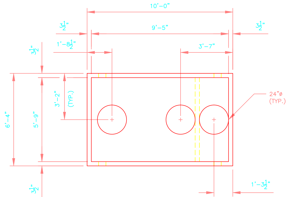
PLAN VIEW
