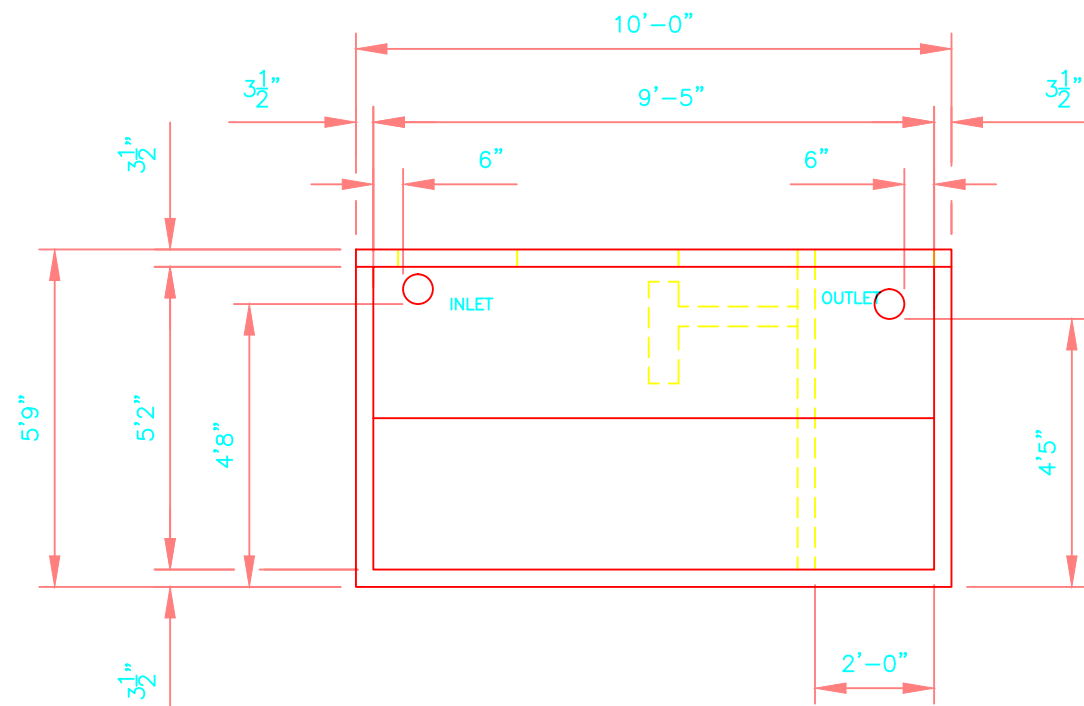
ELEVATION VIEW
