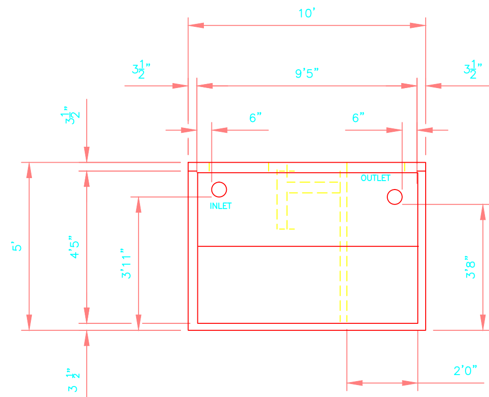
ELEVATION VIEW
