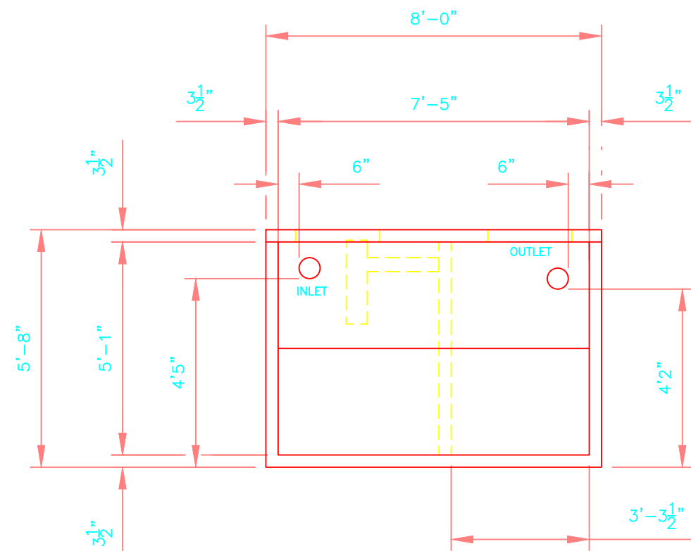
ELEVATION VIEW
